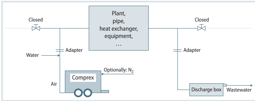
Fig. 1. Diagram of Complex cleaning in the industrial field. The method works by the pulsed charging of compressed air into a defined cleaning section Source: Hammann; graphic: © Hanser
