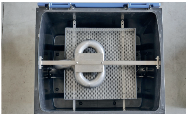
Fig. 2. A manufacturer of preforms for PET bottles used an MCU-300-series Complex unit and a corresponding decompression box © Hammann
